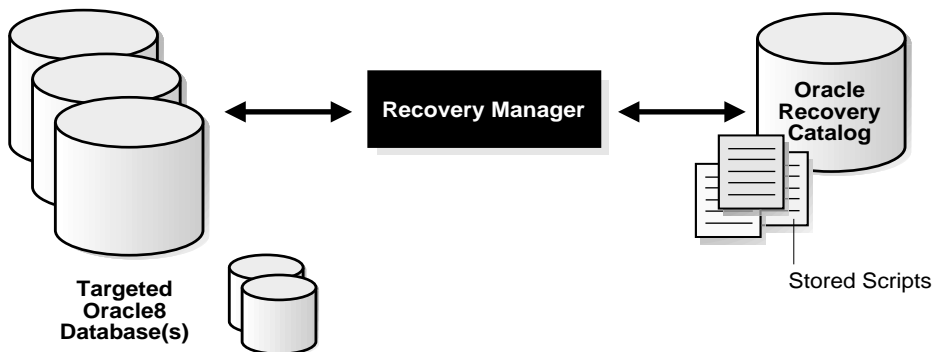
Figure 7-3 Recovery Manager Stored Scripts
