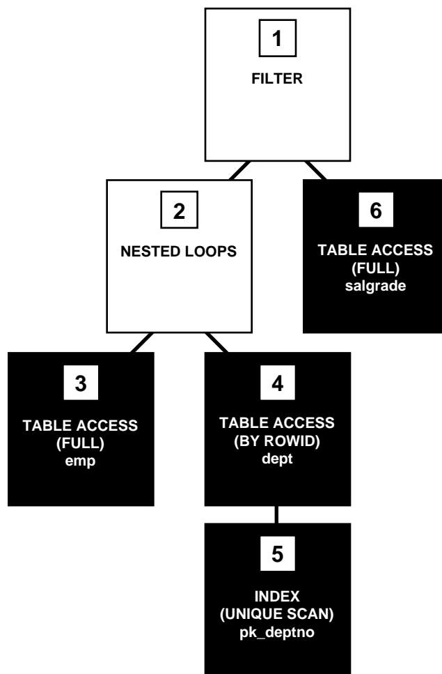
Figure 20–1 An Execution Plan
