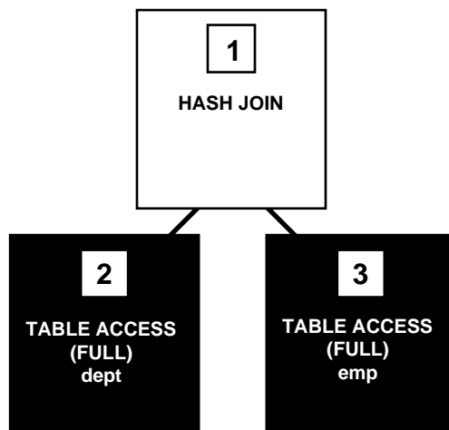
Figure 20–14 Hash Join
