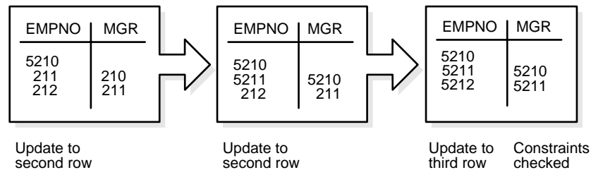
Figure 24–9 Constraint Checking
