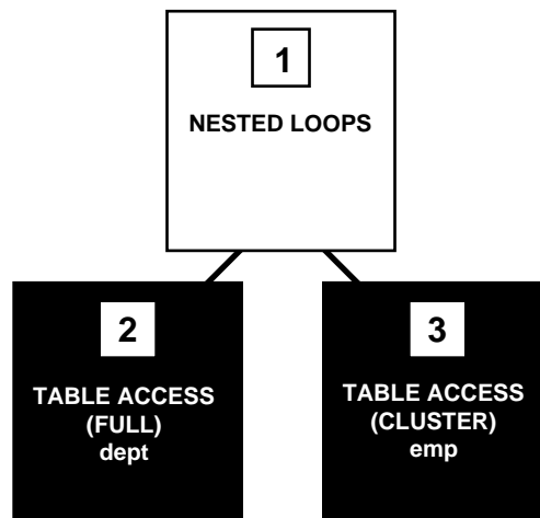
Figure 20–13 Cluster Join
