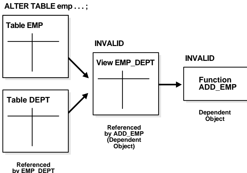
Figure 19–2 Indirect Dependencies
