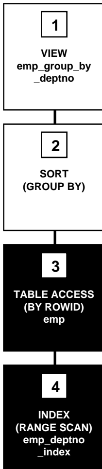
Figure 20-5 Accessing a View Defined with a GROUP BY Clause
